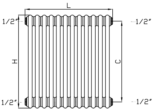
4 Column Front View
